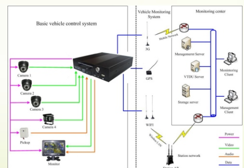
BUSWAY CCTV SYSTEM SKETCH
