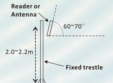
Installation Drawing on the Spot
